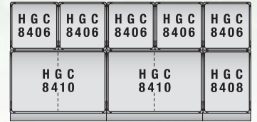
UNIT 12-2 幅3,150mm/高さ1,570mm
